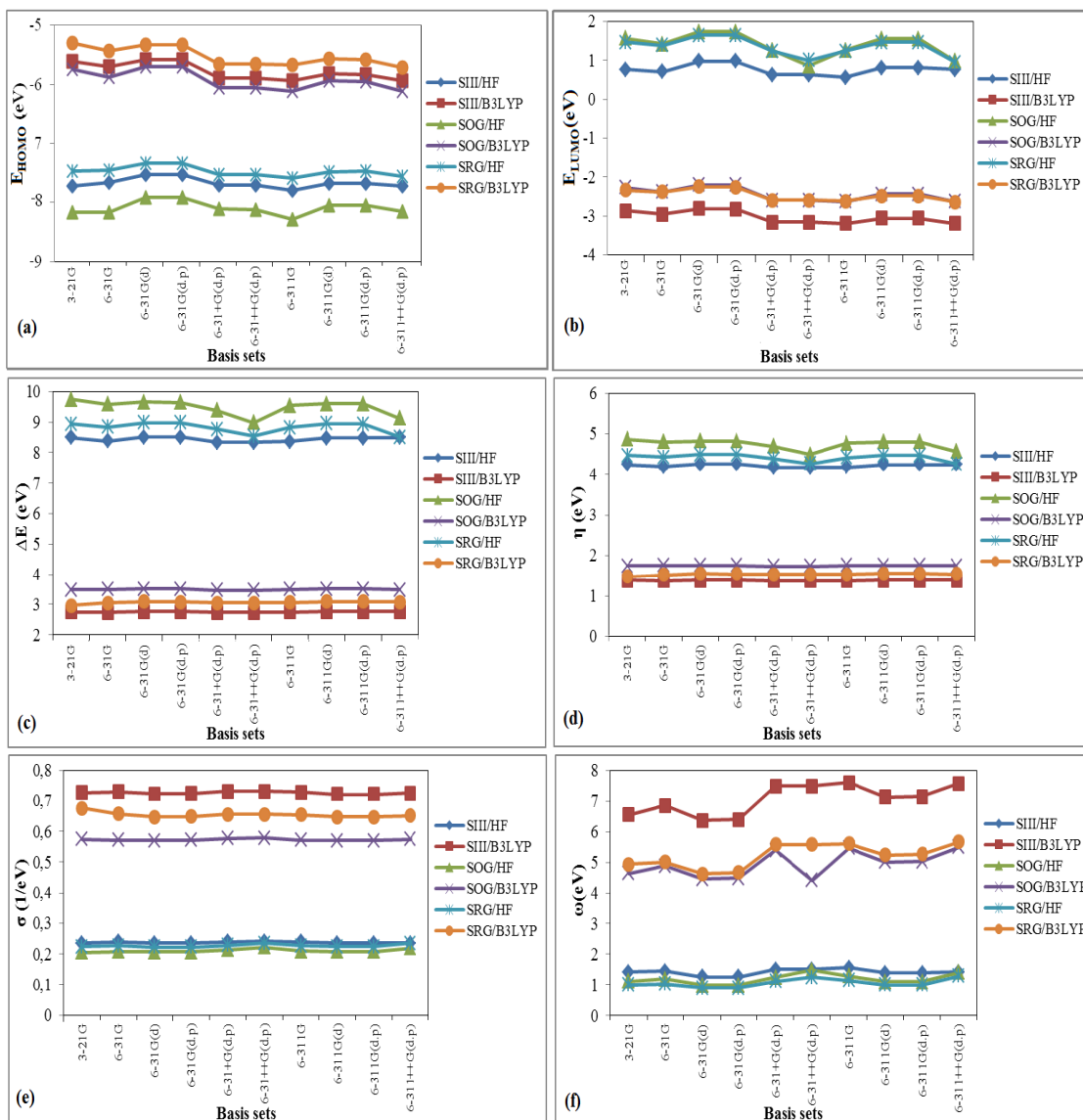
Fig. 5. Variation of (a) E_{HOMO} (eV) (b) E_{LUMO} (eV) (c) HOMO-LUMO energy gap ( \Delta E , in eV) (d) hardness ( \eta , in eV) (e) softness ( \sigma , in 1/eV) (f) global electrophilicity index ( \omega , in eV) of sudan dyes with HF and B3LYP methods and different basis sets.
