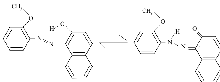
Fig 2. Tautomeric equilibrium for the SRG.
