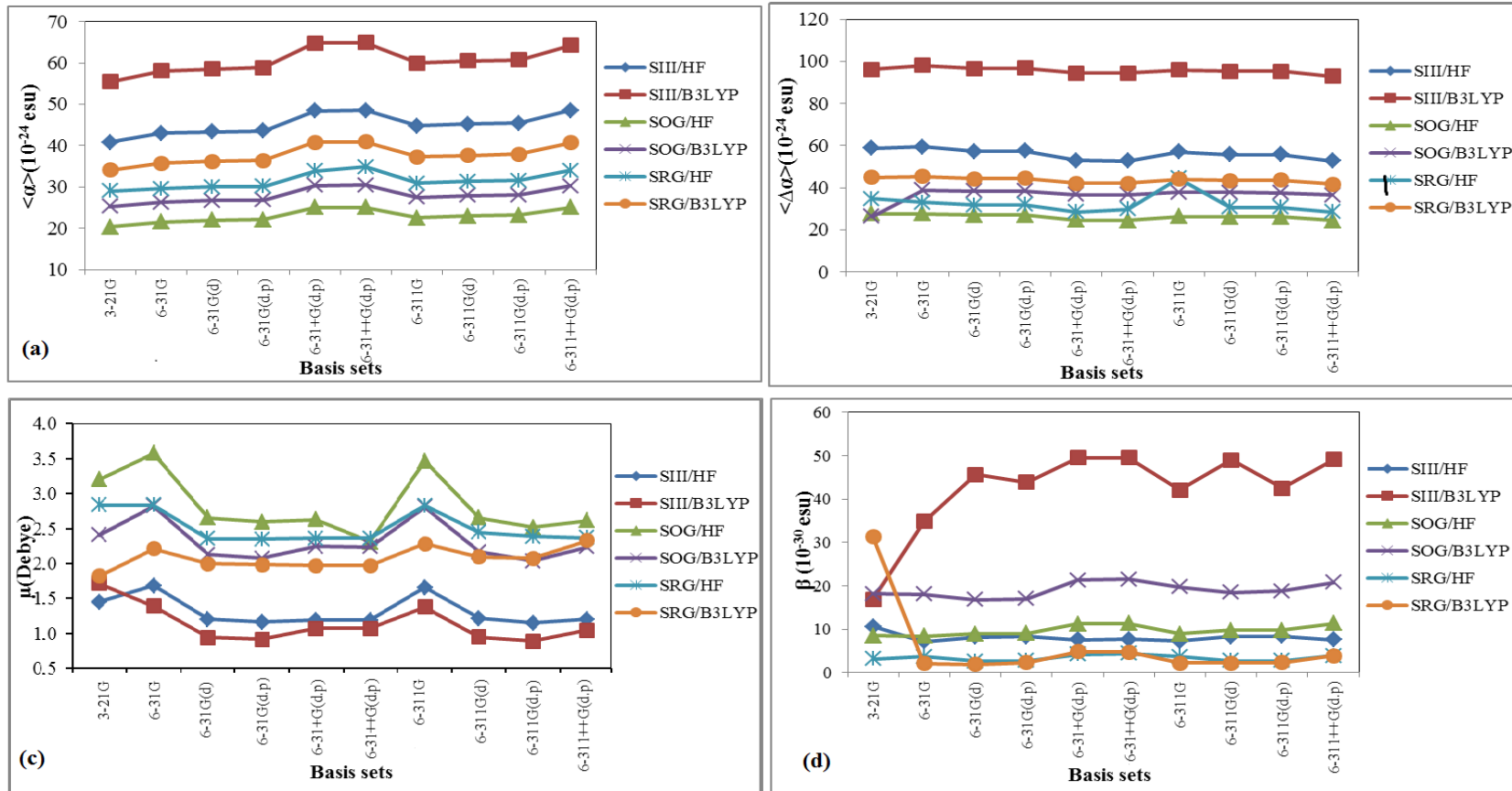
Fig. 6. Variation of (a) polarizability ( \langle\alpha\rangle , in 10^{-24} esu) (b) the anisotropy of the polarizability ( \langle\Delta\alpha\rangle , in 10^{-24} esu) (c) ground-state
