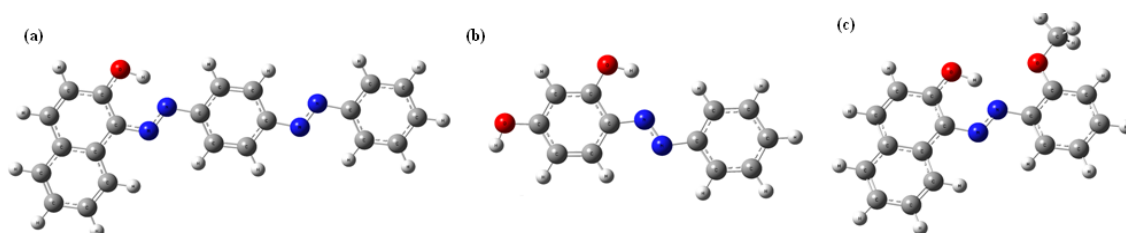
Fig. 3. The optimized structures obtained using B3LYP/6-31G(d,p) level of (a) SIII, (b) SOG and (c) SRG.
